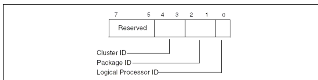
Figure 7-5. Interpretation of the APIC ID
