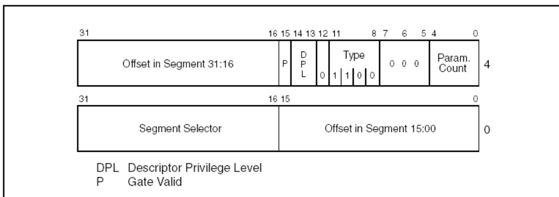
Figure 4-7. Call-Gate Descriptor
