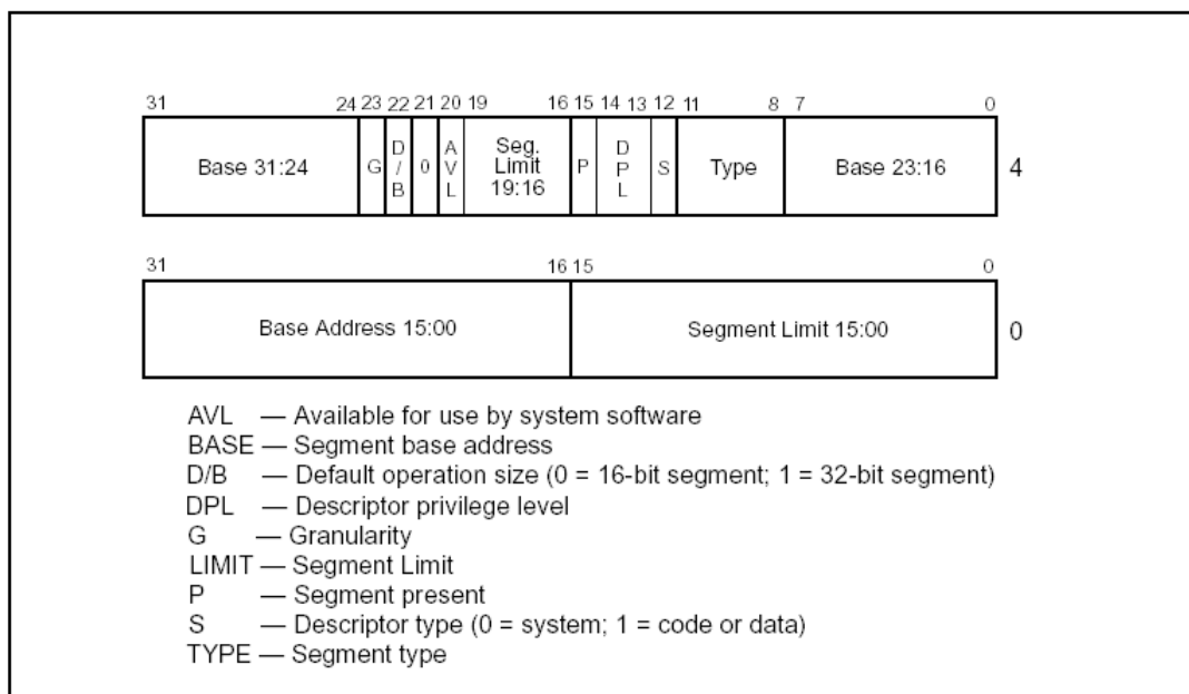
Figure 3-8. Segment Descriptor
