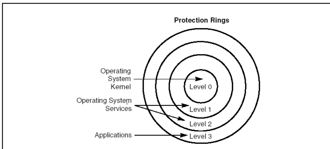
Figure 4-2. Protection Rings
